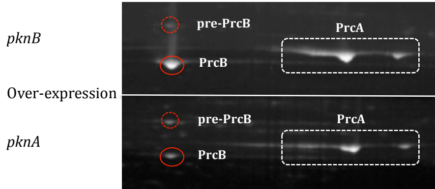
Fig. 2.5: PknA affects the integrity of the proteasome core complex in mycobacteria. Proteasome purified from M. smegmatis containing pknA - or pknB -overexpressing constructs was analyzed using 2D-PAGE and flamingo staining. Top panel: purification from cells with pknB , bottom panel: purification from cells with pknA . PrcA-strep (dotted box), pre-PrcB (dotted red circle), and processed PrcB (red circle) are shown.
